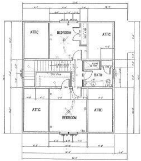
SECOND FLOOR PLAN SCALE 3/8"=1'-0"
