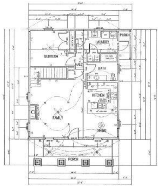
FIRST FLOOR PLAN SCALE 1/4"=1'-0"
